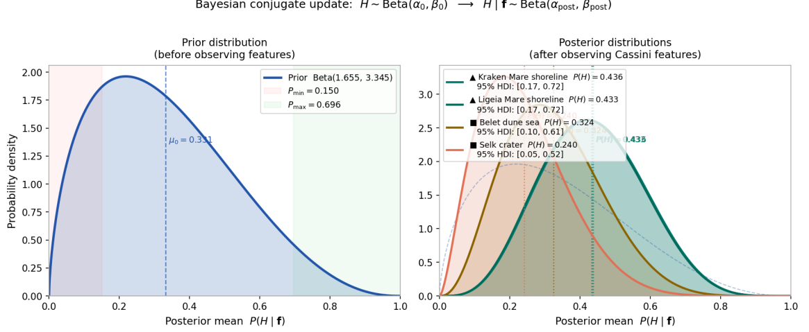
Figure 2.2: Beta-conjugate Bayesian update for four representative Titan surface environments. Left: the prior distribution H \sim \text{Beta}(1.655, 3.345) with mean \mu_0 = 0.331 . Shaded bands mark the hard bounds [P_{\min}, P_{\max}] = [0.150, 0.696] . Right: posterior distributions after incorporating the Cassini feature vector \mathbf{f} for each site (parameters \kappa = 5 , \lambda = 6 ; present epoch). The update sharpens and shifts each distribution in proportion to how far the site’s weighted feature sum \sum_i w_i f_i departs from the prior mean. Polar lake shores (cyan) shift markedly right; the equatorial crater (red) shifts left; the dune sea (amber) remains near the prior. 95% HDI values are given in the legend.
